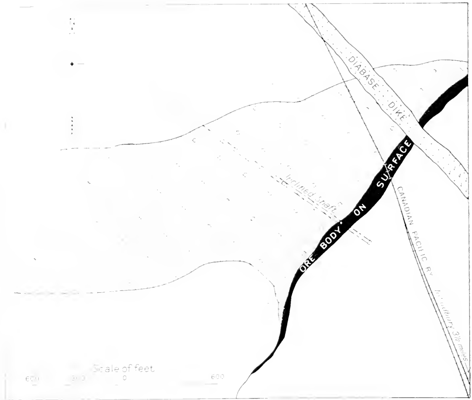
Fig. 51—Map showing Murray ore body, Sudbury area, Ontario. The shaded area denotes the known extent of the deposit below the surface; the ore body dips to the northwest at an angle of 36° as shown in Fig. 52. The small circles indicate diamond drill holes. From drawing by the British America Nickel Corporation.
